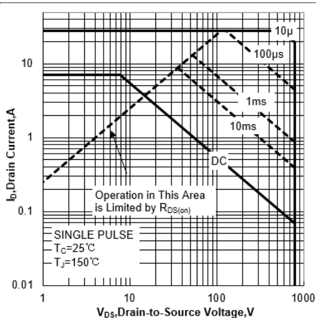
Figure 1b Safe Operating Area (FullPAK)
