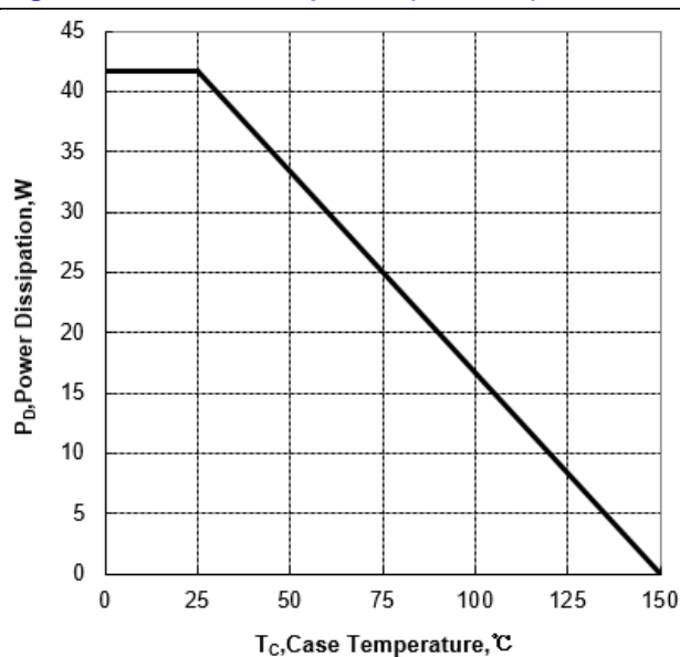
Figure 2b Power Dissipation (FullPAK)
